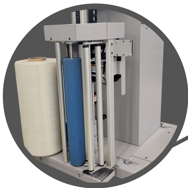
New Redesigned Lightweight Carriage
